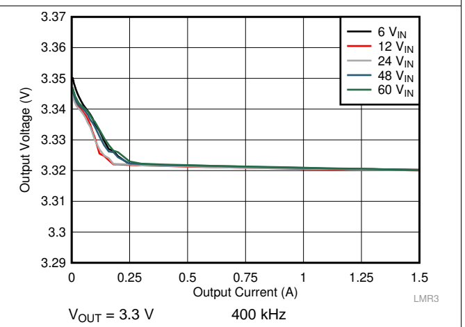
Figure 25. Load Regulation
