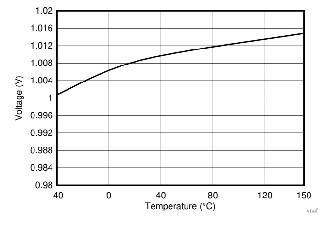
Figure 5. Reference Voltage Drift
