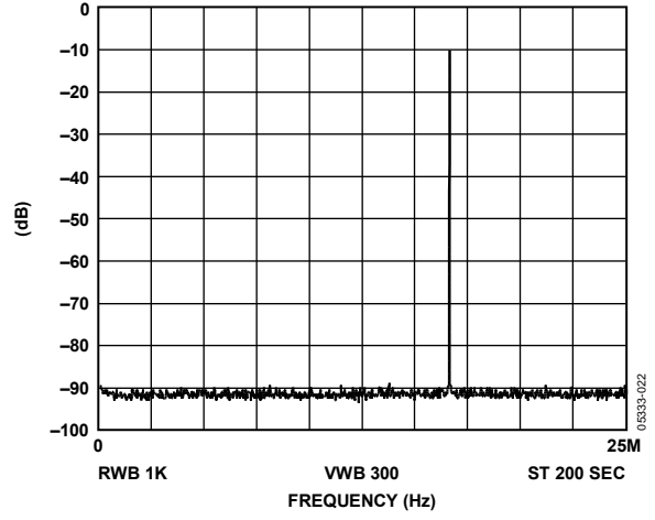
Figure 30. f_{MCLK} = 50 \text{ MHz} ; f_{OUT} = 16.667 \text{ MHz} = f_{MCLK}/3 , Frequency Word = 5555555
