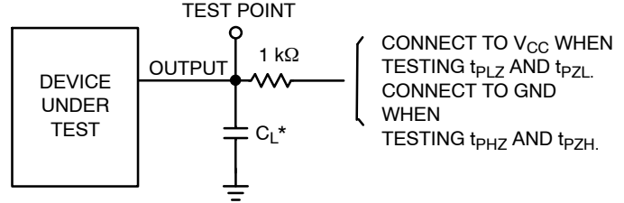
Figure 6. Test Circuit
