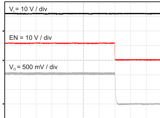
Figure 45. TPS563209 Shut Down Relative to EN
