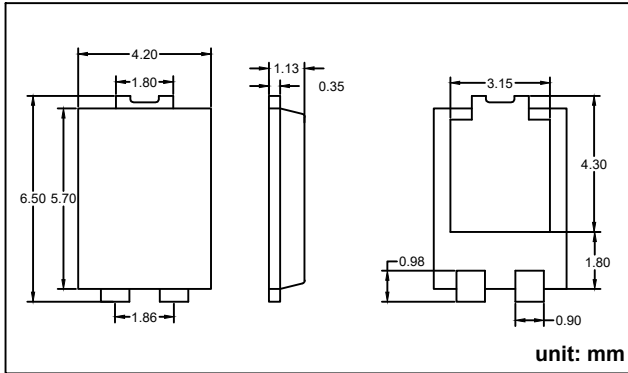
TO-277B(EOL)
