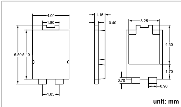
TO-277(Replacement)
