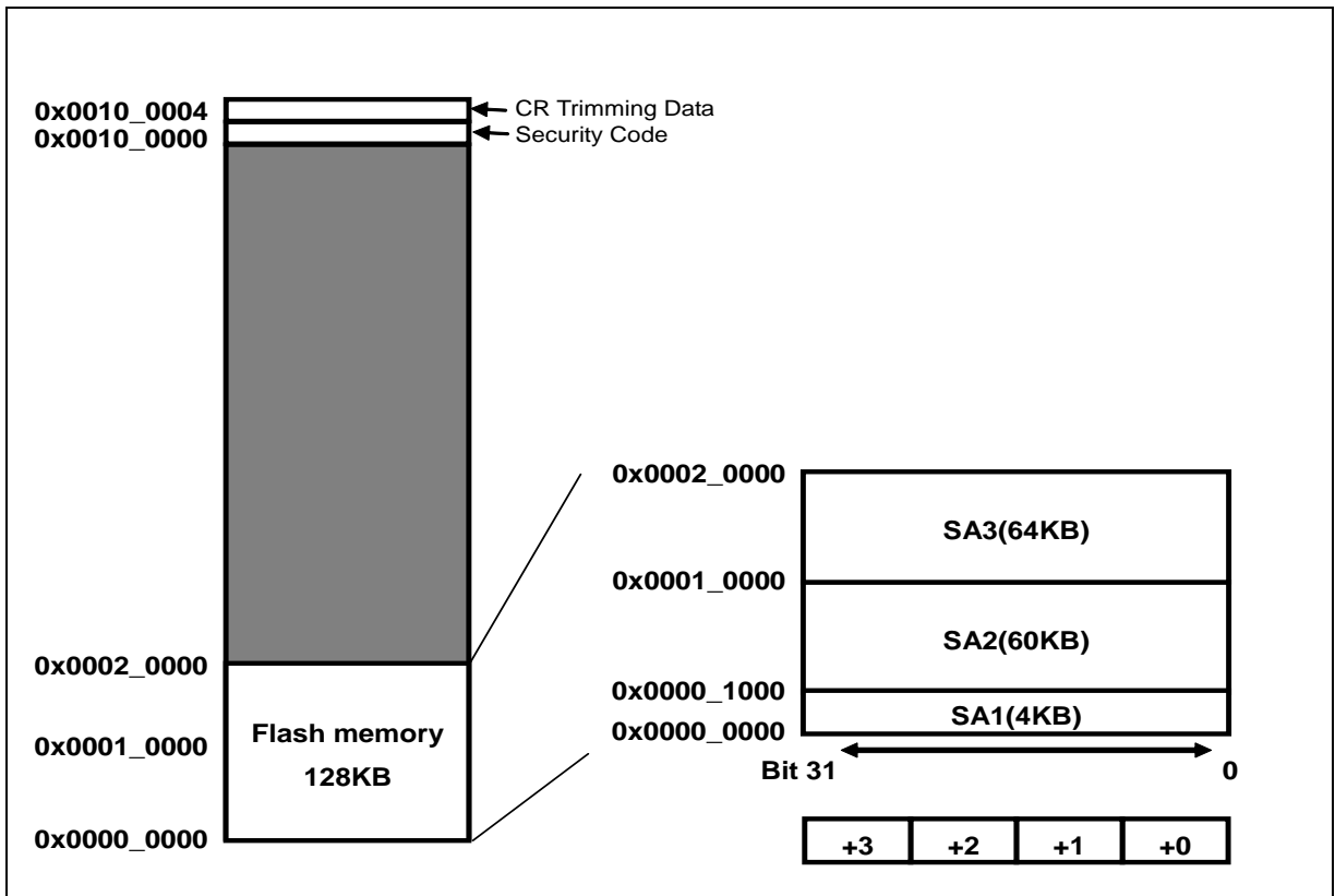
Figure 1-2. Memory Map of the MB9AF132/MB9AFA32/MB9AF1A2/MB9AFAA2 Flash Memory
