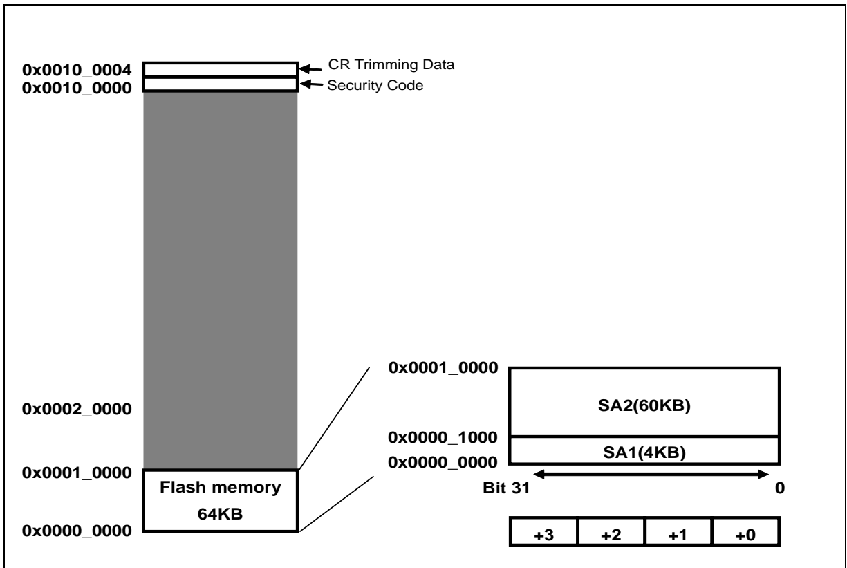
Figure 1-1. Memory Map of the MB9AF131/MB9AFA31/MB9AF1A1/MB9AFAA1 Flash Memory
