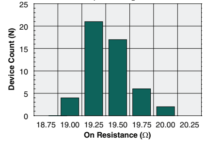
Typical On-Resistance Distribution (N=50, I F =5mA, I L =120mA)
