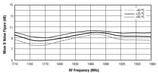
Figure 12. Mixer B Noise Figure vs Frequency and Temperature
