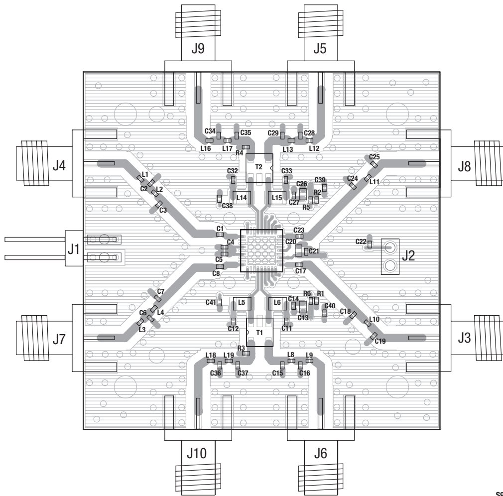
Figure 35. SKY73023-11 Evaluation Board Assembly Diagram
