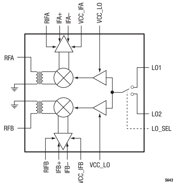
Figure 1. SKY73023-11 Block Diagram
