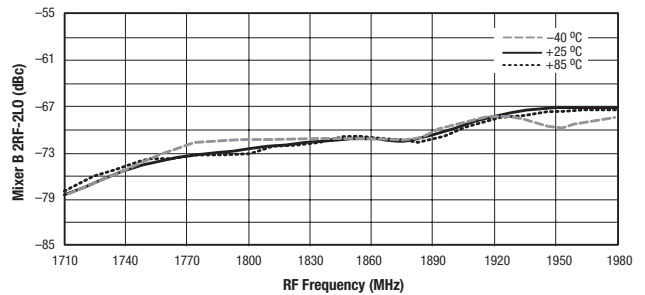
Figure 26. Mixer B 2RF-2LO vs Frequency and Temperature
