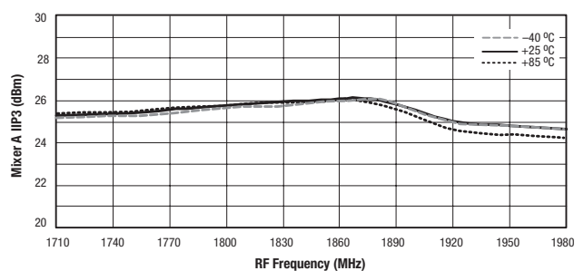
Figure 14. Mixer A IIP3 vs Frequency and Temperature
