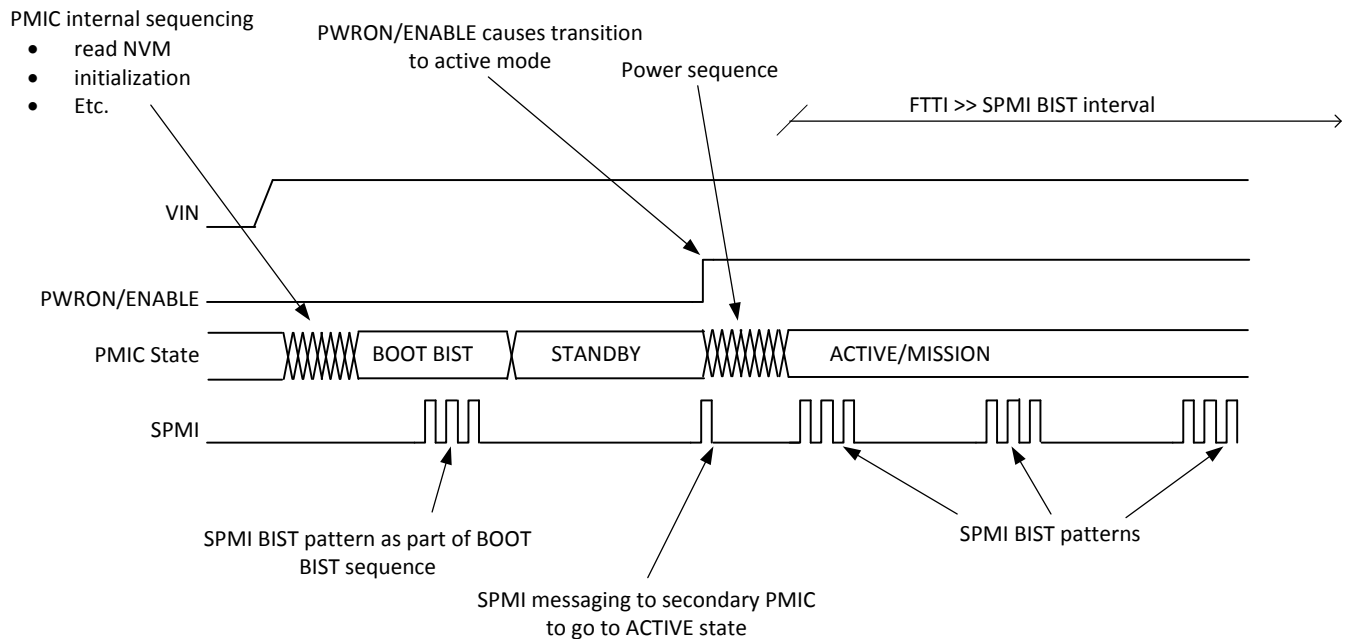
Figure 8-50. SPMI-BIST Operation
