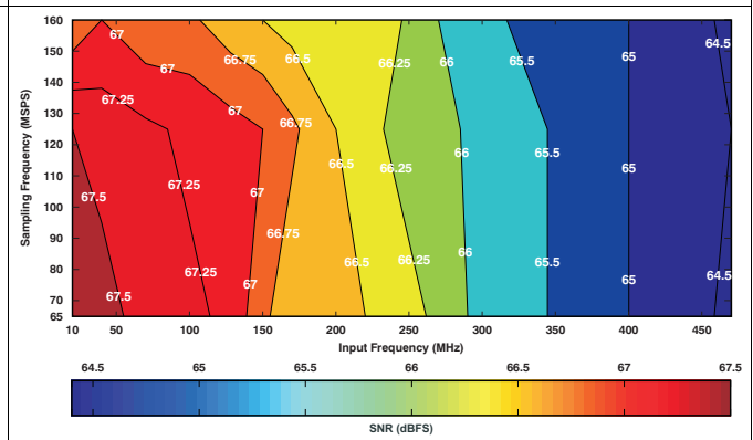
Figure 132. ADS424x Signal-to-Noise Ratio (6-dB Gain)
