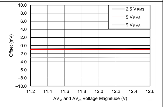
Figure 17. Offset vs Supply Voltage
