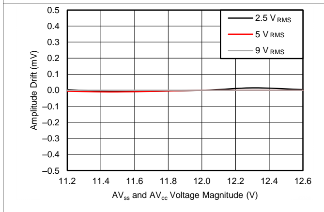
Figure 16. Amplitude Drift vs Supply Voltage
