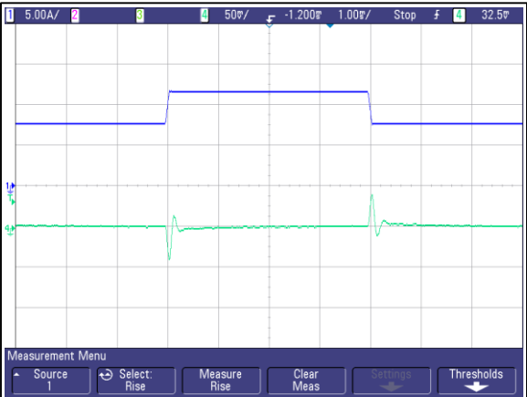
Figure 7: AVD50B-48S3V3 Transient Response (1mS/div) 0.1A/us slew rate Ch 4: Vo (50mV/div) Ch 1: Io (5A/div)
