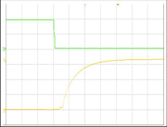
Figure 5: AVD50B-48S3V3 Remote ON Waveform (10mS/div) Ch 1: Vo (1V/div) Ch 2: Remote ON (2V/div)
