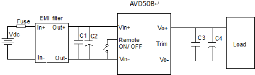
Figure 17 Typical application
