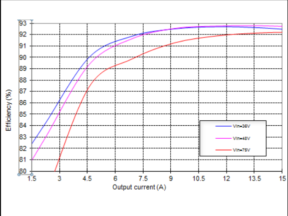
Figure 9: AVD50B-48S3V3 Efficiency Curves @ 25 degC Loading: Io = 10% increment to 15A
