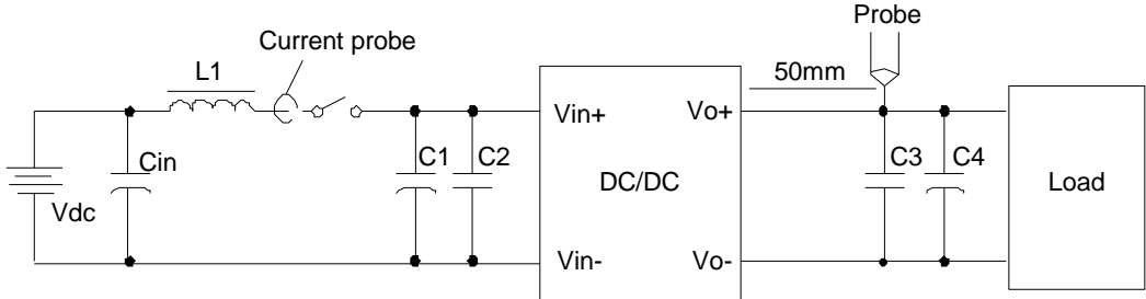
Figure 21 Input ripple & output ripple & noise test configuration
