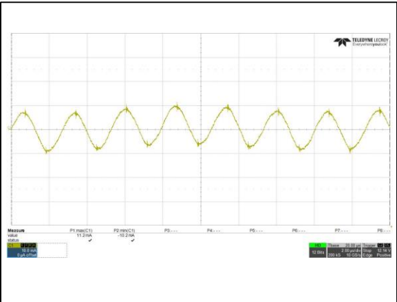
Figure 1: AVD50B-48S3V3 Input Reflected Ripple Current Waveform Ch 1: Iin (2uS/div, 10mA/div)
