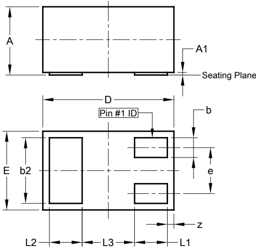
X1-DFN1006-3
