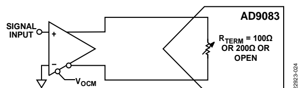
Figure 61. DC-Coupled Inputs to the AD9083 Using an Amplifier (Note the V_{CM} Pin Providing the Common-Mode Voltage)
