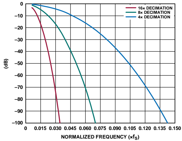
Figure 79. Zoomed in Image of the CIC Filter Response Shown in Figure 78; Normalized to f_s
