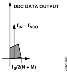
Figure 74. Output Spectrum of the FIR Filter Output of a Baseband Signal
