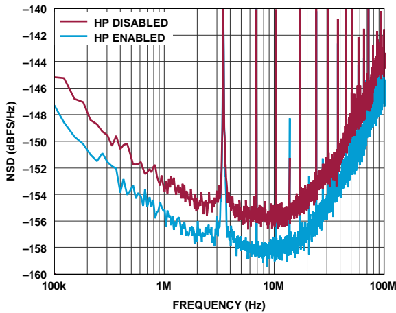
Figure 11. ADC NSD with and Without EN_HP, 2 GSPS
