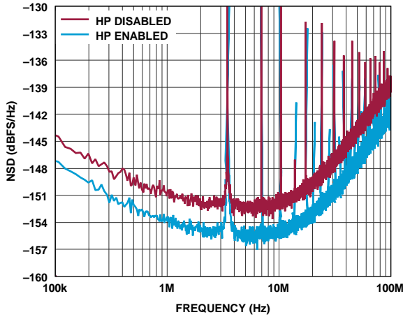
Figure 10. ADC NSD with and Without EN_HP, 1 GSPS
