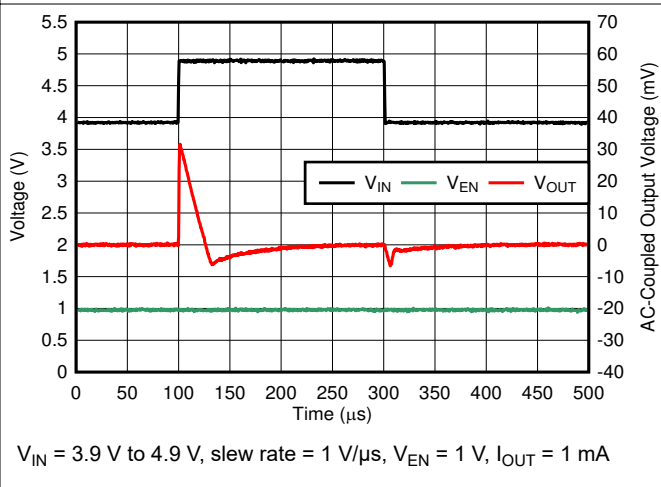
Figure 6-18. Line Transient
