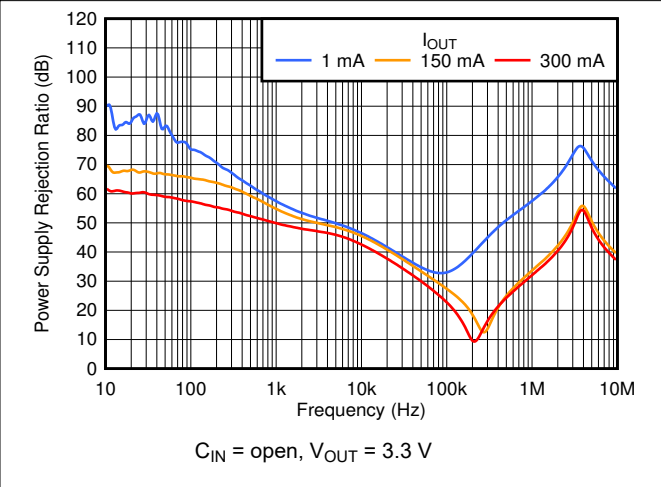
Figure 6-16. PSRR vs Frequency and I_{OUT}
