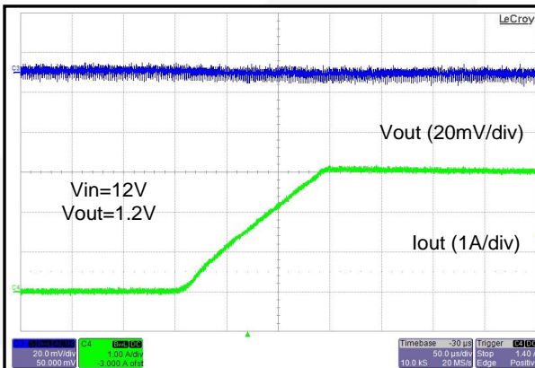
Figure 23. FAN23SV06P Operation as Load Changes from 0 A to 3 A
