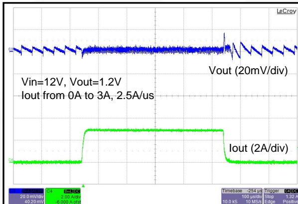
Figure 26. FAN23SV06 Load Transient from 0% to 50% Load Current
